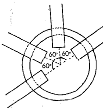
Figure 2. 4-hole joint from above.
