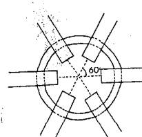
Figure 1. 6-hole joint from above.
